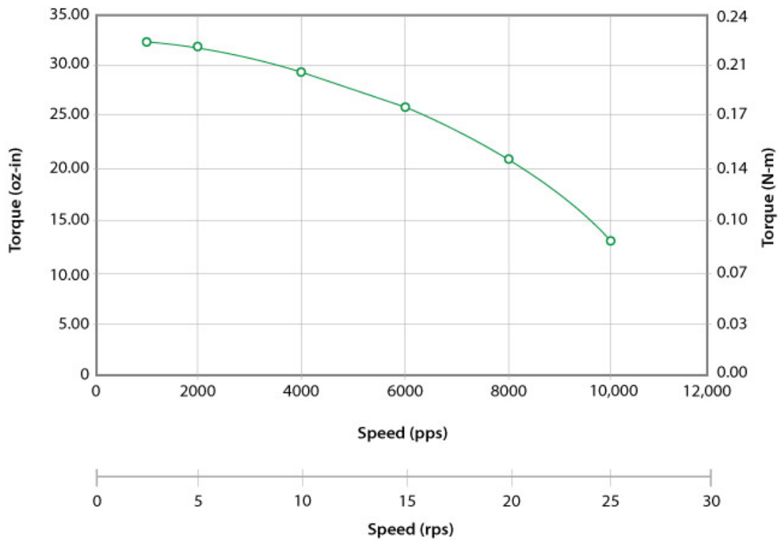
G4518S-01 24VDC, 1.5 Amps/Phase, Bipolar, 1/2 Stepping
